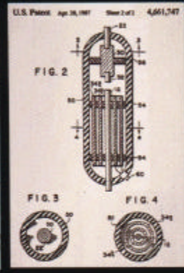
Conversion Tube Patent
